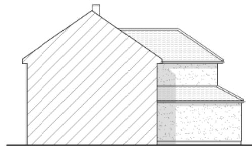
PROPOSED RIGHT FLANK ELEVATION
